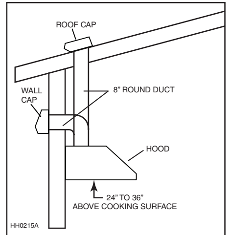
MODEL iQ6 (SINGLE) INTERIOR BLOWER 8" ROUND DUCTWORK
