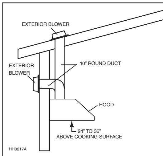
MODEL EB9 OR EB15 EXTERIOR BLOWER TYPICAL DUCTWORK
