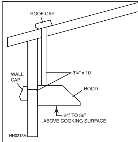
MODEL P5 (SINGLE) INTERIOR BLOWER TYPICAL RECTANGULAR DUCTWORK
