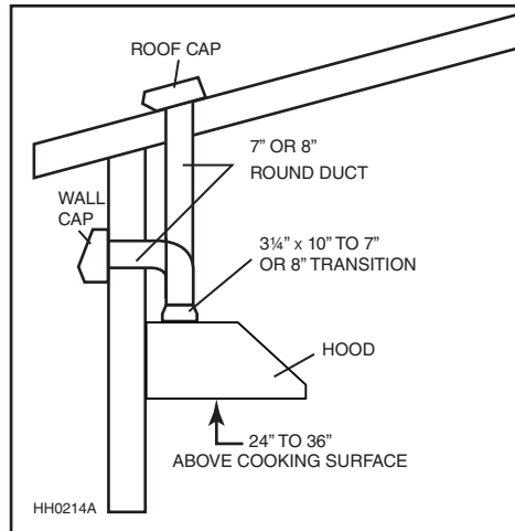
MODEL P5 (SINGLE) INTERIOR BLOWER 7" OR 8" ROUND DUCTWORK
