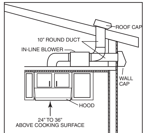
MODEL ILB6, ILB9 OR ILB11 IN-LINE BLOWER TYPICAL DUCTWORK
