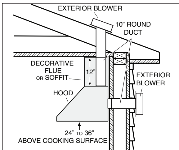
MODEL EB9 OR EB15 EXTERIOR BLOWER TYPICAL DUCTWORK
