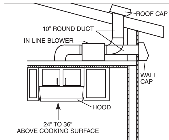
MODEL ILB6, ILB9 OR ILB11 IN-LINE BLOWER TYPICAL DUCTWORK
