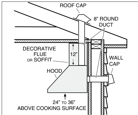
MODEL iQ6 SINGLE INTERIOR BLOWER TYPICAL DUCTWORK
